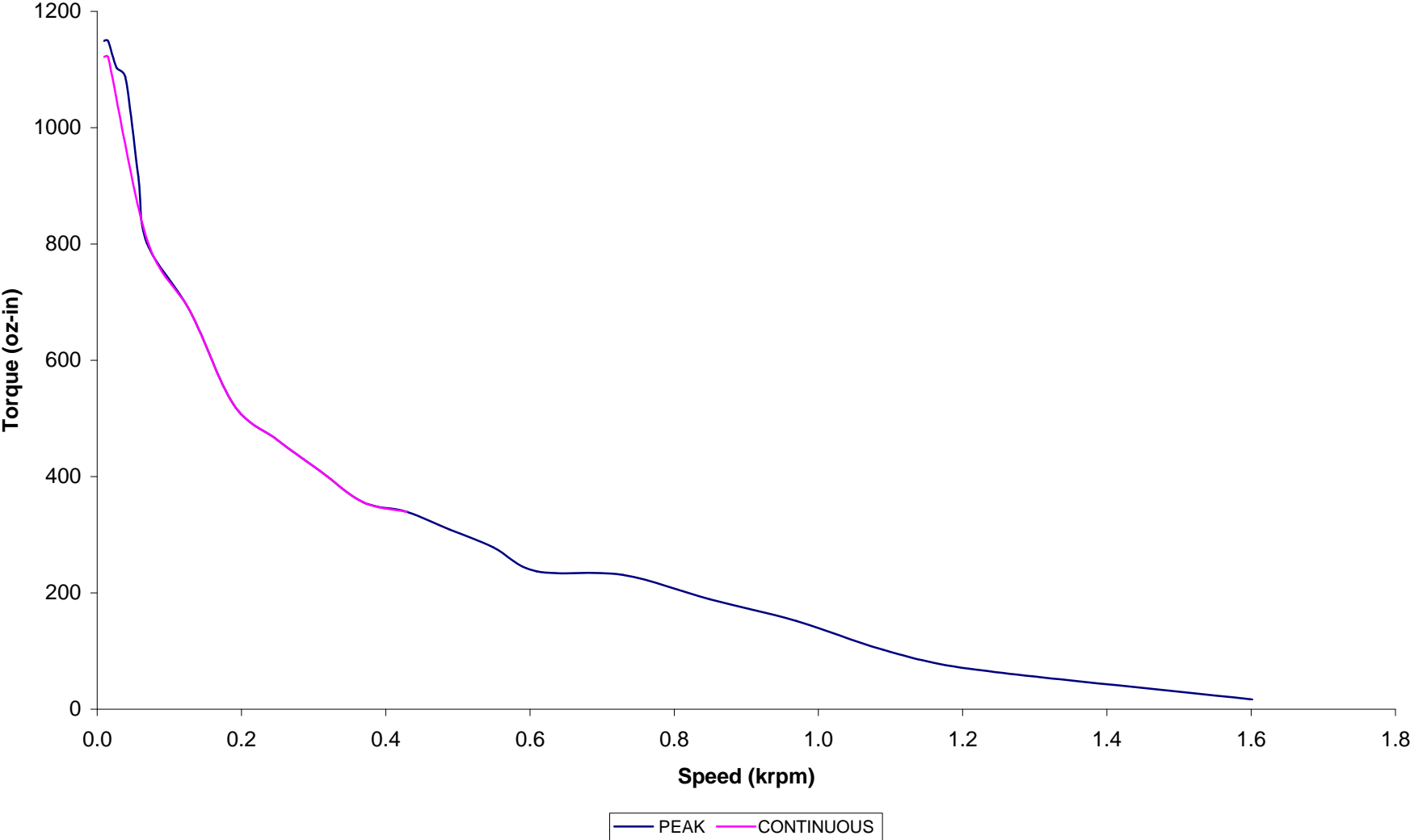
ST3430 Torque vs. Speed (75 VDC) using a PS75V6AF power supply (10% Derated Torque)
