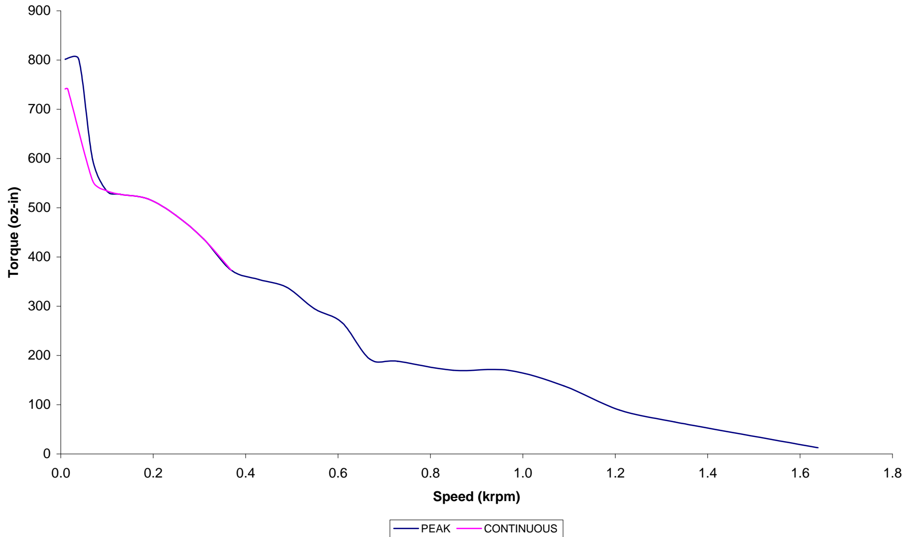
ST3420 Torque vs. Speed (75 VDC) using a PS75V6AF power supply (10% Derated Torque)
