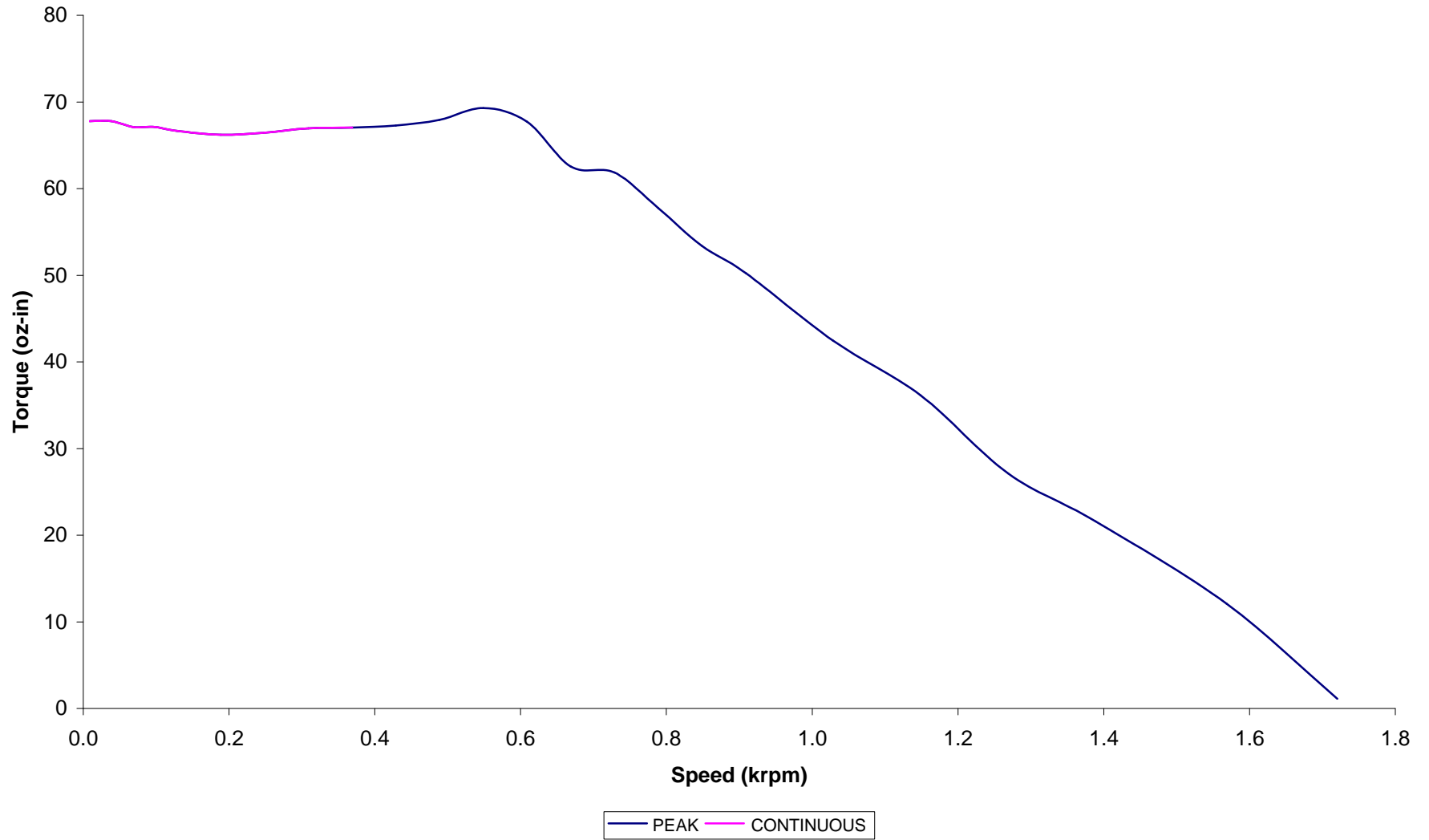
ST2310 Torque vs. Speed (75 VDC) using a PS75V6AF power supply (10% Derated Torque)
