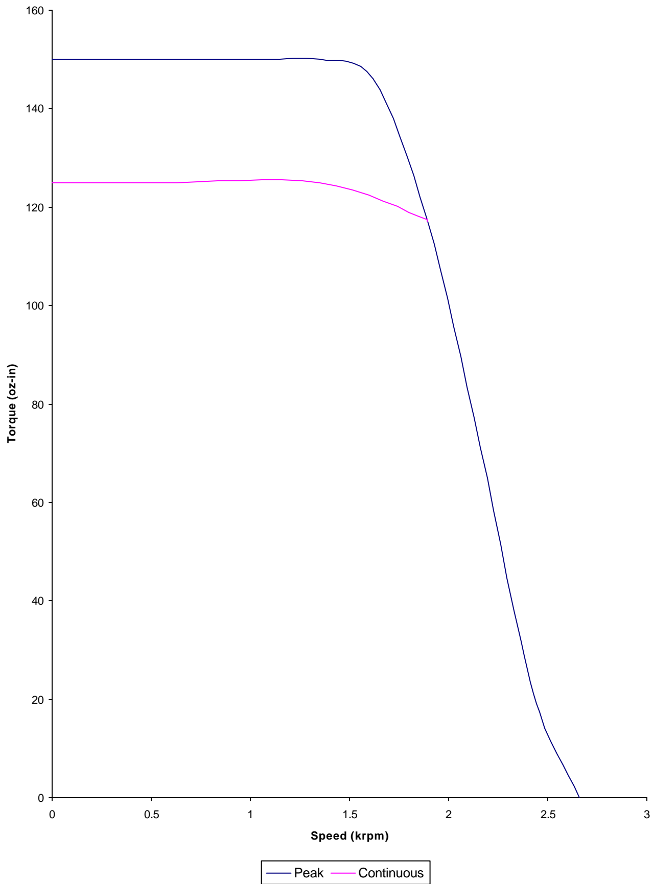
SM3416D Torque vs. Speed at 42 VDC using a PS42V20AF supply
